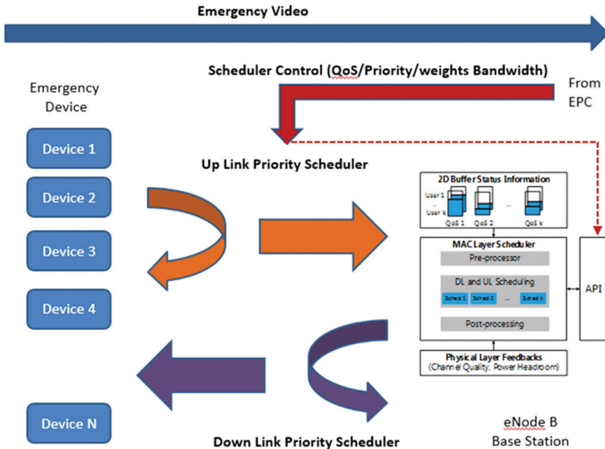
Figure 23.2 Scheduler overview.
