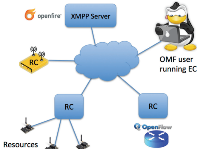
Figure 12.3 OMF 6 architecture.
