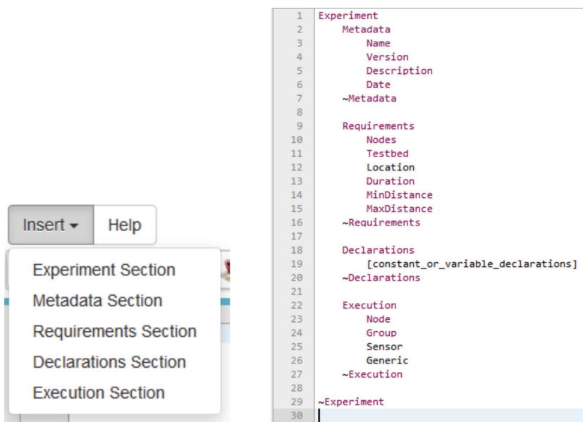
Figure 15.4 An example of inserting code templates in the textual editor.
