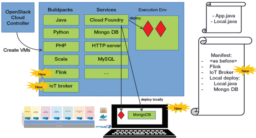
Figure 24.1 PaaS deployment extended for IoT in WAZIUP.
