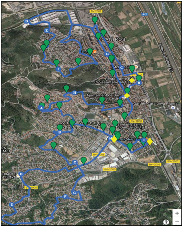
Figure 7.9 Routes followed by the bus and location of the sensor units: low-power wake-up (green) and Airbase air quality (yellow) devices.
