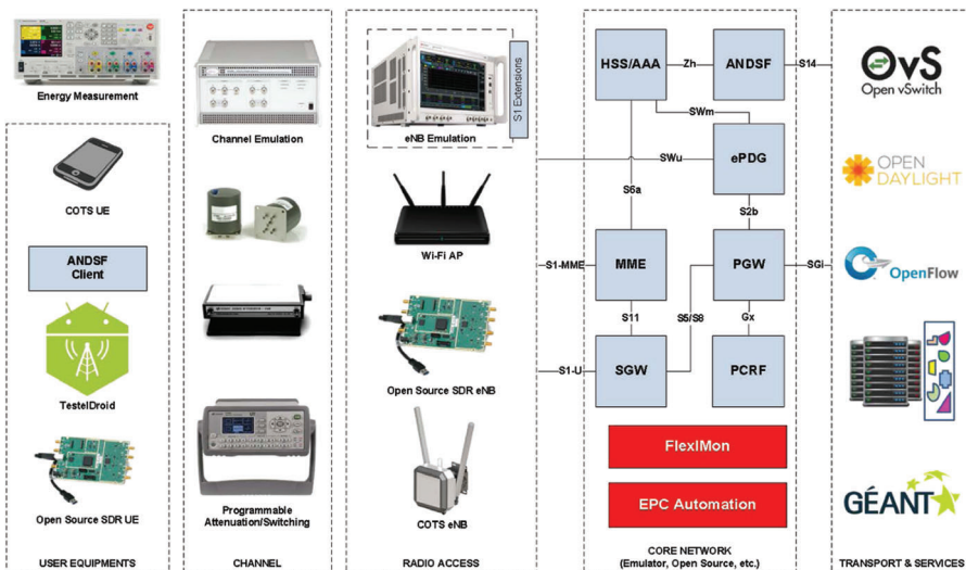
Figure 6.1 PerformNetworks architecture.
