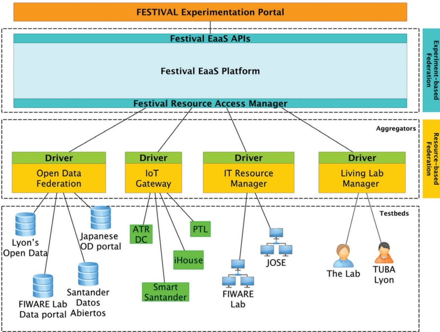
Figure 28.1 FESTIVAL architecture.
